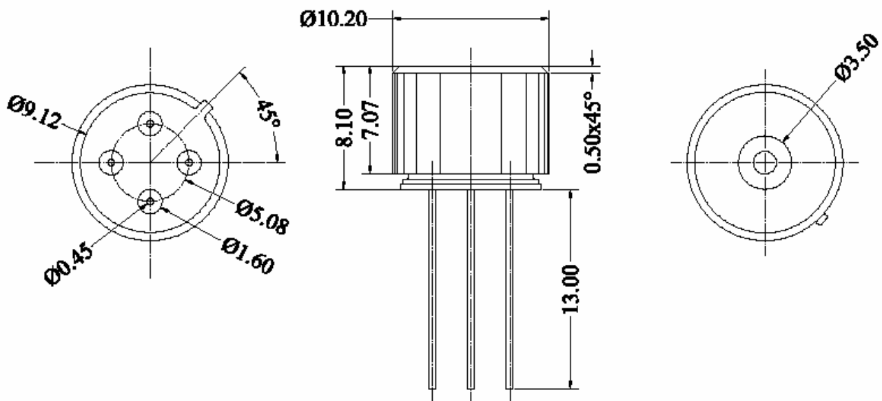
Figure 30: MLX90614XCC package
